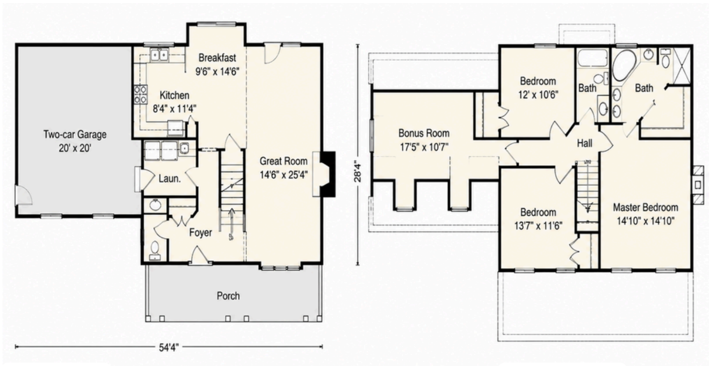
First Floor
